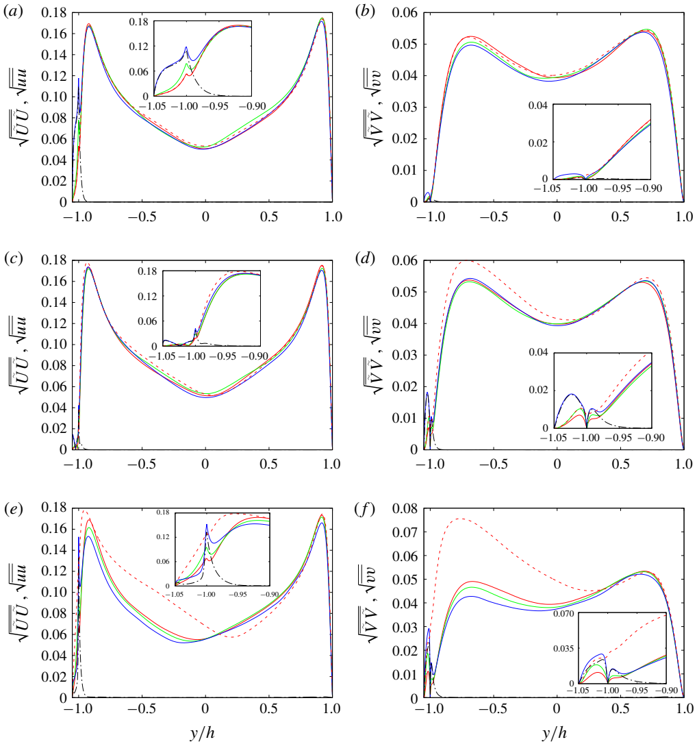
FIGURE 10. (Colour online) Root mean square of streamwise velocity (left) \sqrt{\overline{uu}} , and wall-normal velocity (right) \sqrt{\overline{vv}} : (a,b) Longitudinal square bars, (c,d) transversal square bars and (e,f) staggered cubes a = 0.875 . Dashed lines one fluid configuration, solid lines for two superposed fluids, —, (red) N = 1 , —, (green) N = 2.5 . For N = 100 both the total stress —, (blue), and its dispersive component — · — \sqrt{\overline{\tilde{U}_i \tilde{U}_j}} are shown. A zoom near the texture is shown in the inset. The velocity fluctuations are normalized with the bulk velocity.
