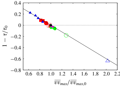
FIGURE 12. (Colour online) Dependence of the amount of drag reduction with the maximum of the wall-normal velocity r.m.s.: ■ longitudinal bars; ● transversal square bars; ▼ staggered cubes with a = 0.5 ; ▲ staggered cubes with a = 0.875 ; solid line, equation (6.8). Empty symbols indicate simulations with only one fluid without interface, solid symbols simulations with two fluids and a slippery interface.
