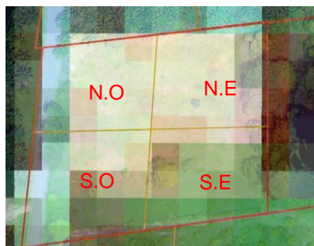
Figura 59. Sector 2.
