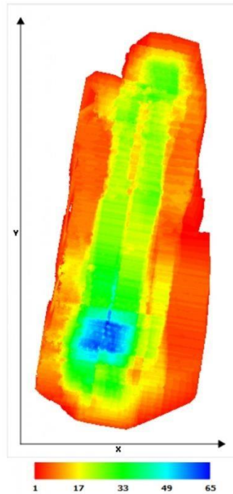
Number of photos seeing the scene: Top view (XY plane) display of the scene, with colors indicating the number of photos that potentially see each area.
